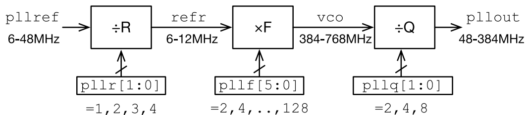
Figure 3: Controlling the FE310-G000 PLL output frequency.
