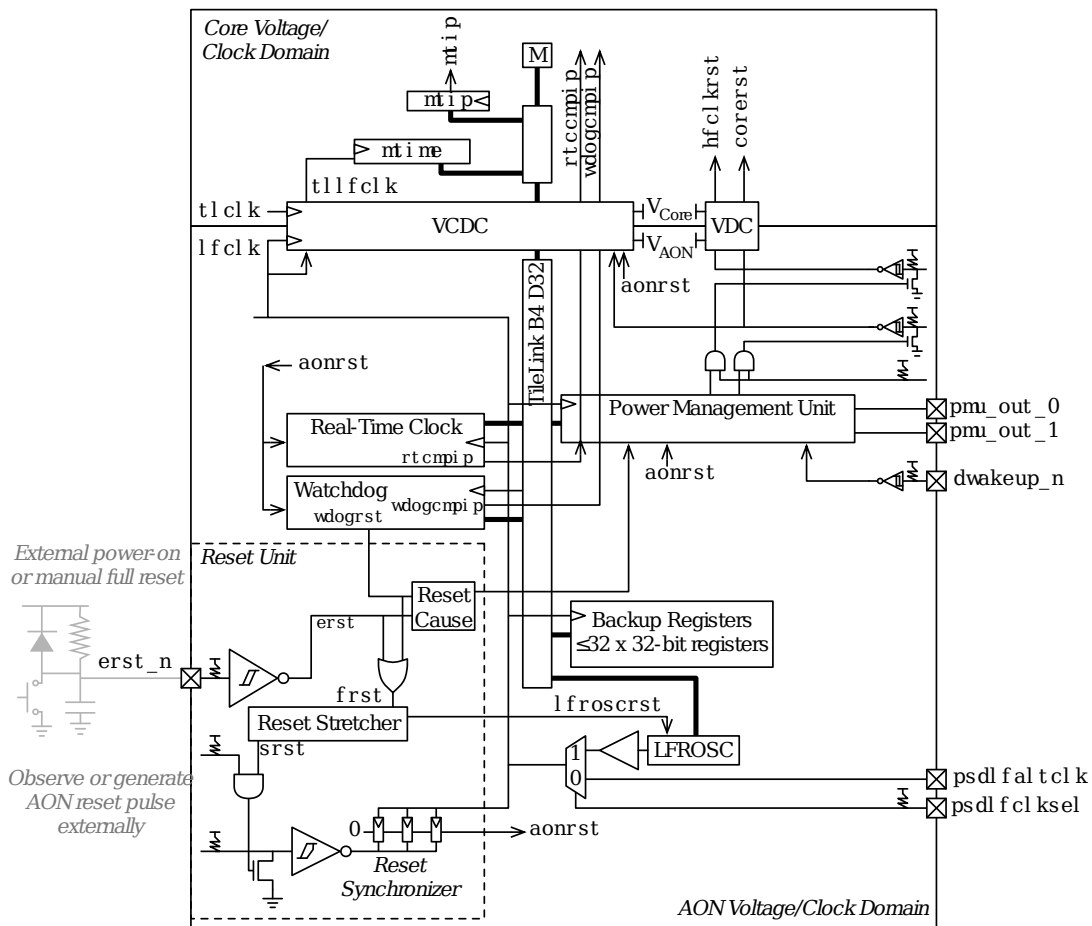
Figure 5: FE310-G000 Always-On Domain
