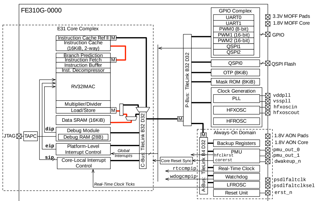
Figure 1: FE310-G000 top-level block diagram.
