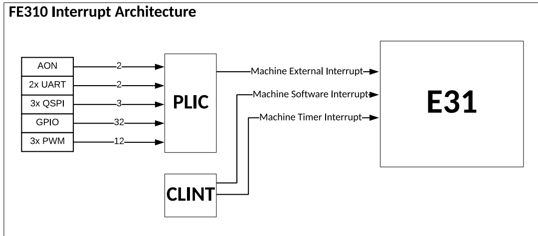
Figure 4: FE310-G000 Interrupt Architecture Block Diagram.
